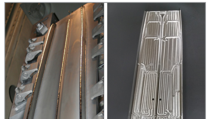
(Above) This photo highlights two different stages of an Airbus rear upper spar that was 3D printed in titanium with Sciaky's EBAM process. The image on the left shows the part in an early preform stage. The image on the right shows the finished part. Courtesy of Sciaky.
