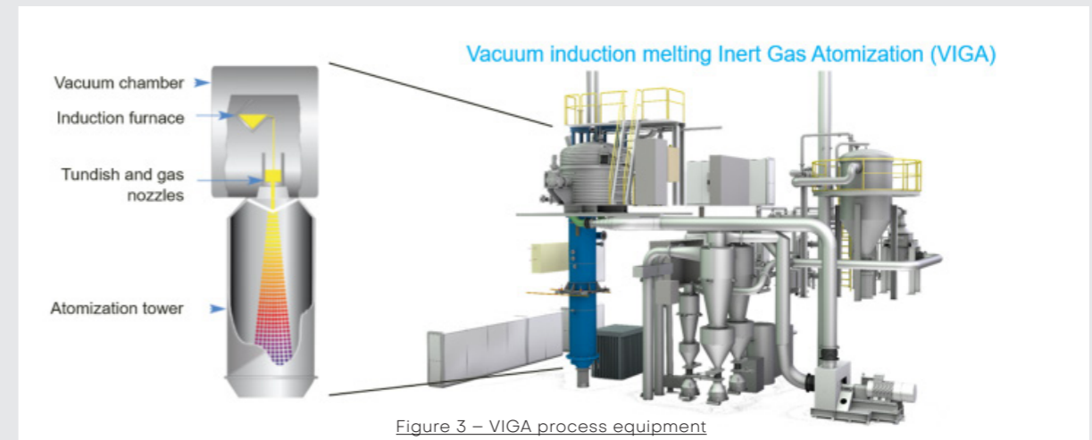
Figure 3 – VIGA process equipment
