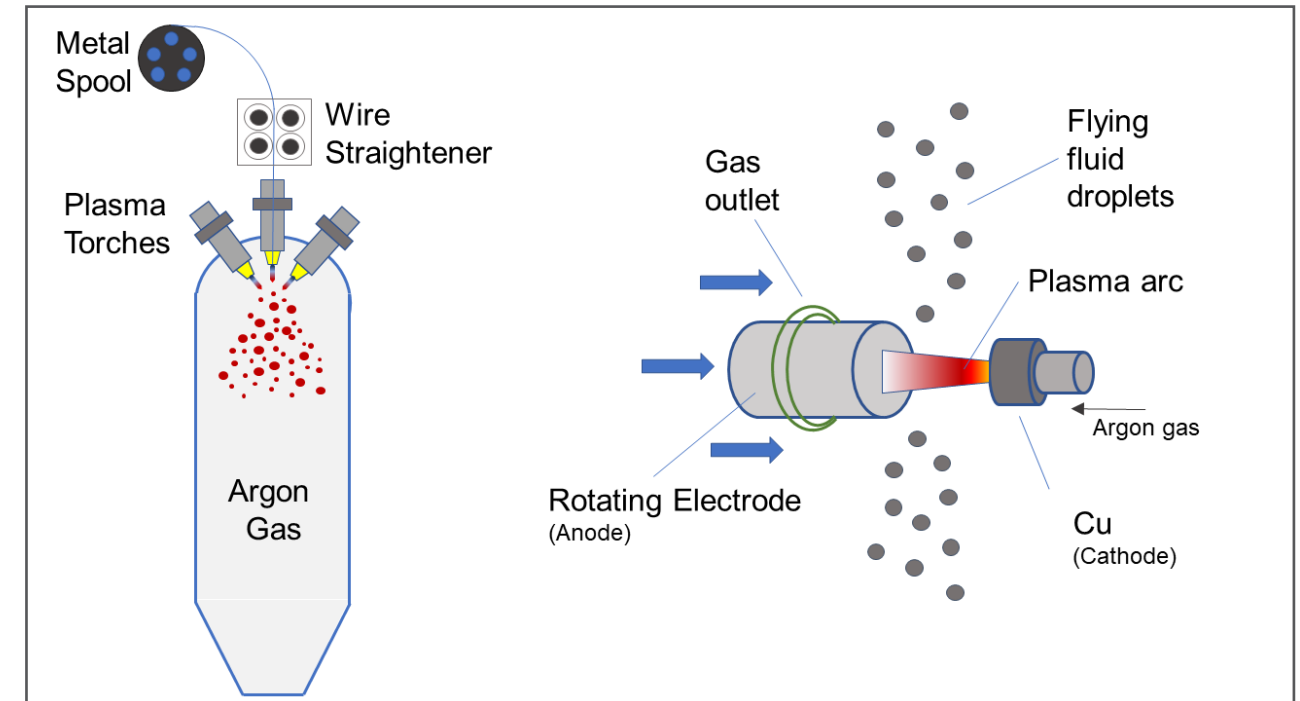
Figure 1: (a) Plasma atomisation (Source: Pyrogenesis) / (b) Plasma Rotating Electrode Process Atomization [7]
