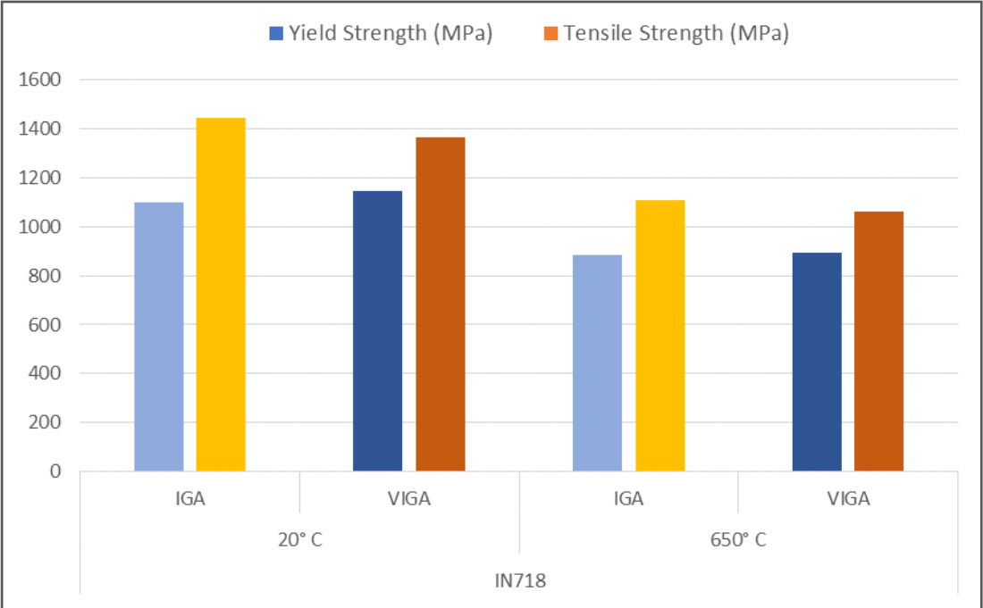
Figure 8: Mechanical properties of Inconel 718 in vertical direction (Solution annealed and aged)
