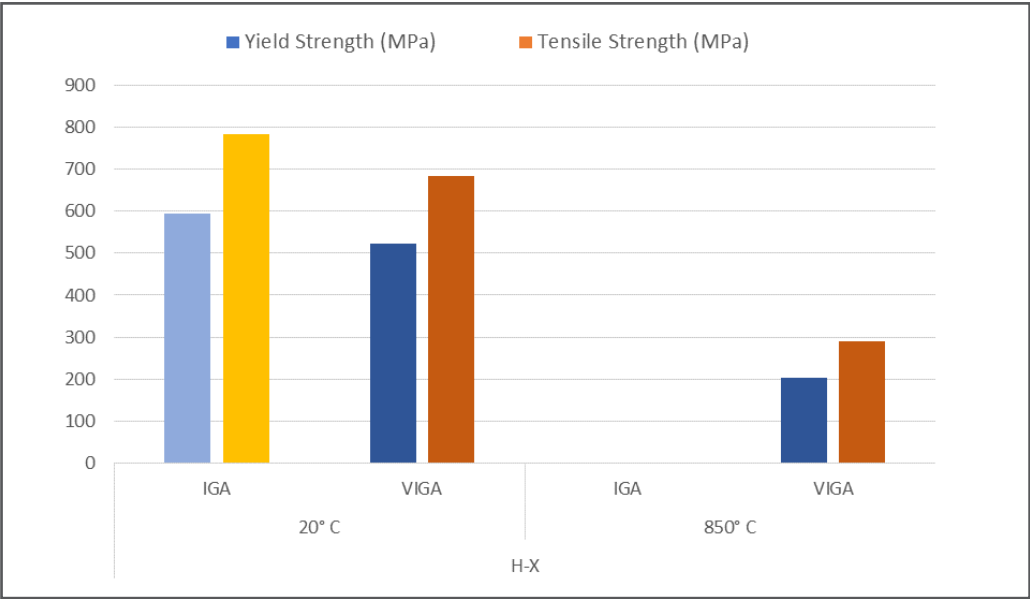
Figure 10: Mechanical properties of H-X alloy in vertical direction (Source: Sandvik)
