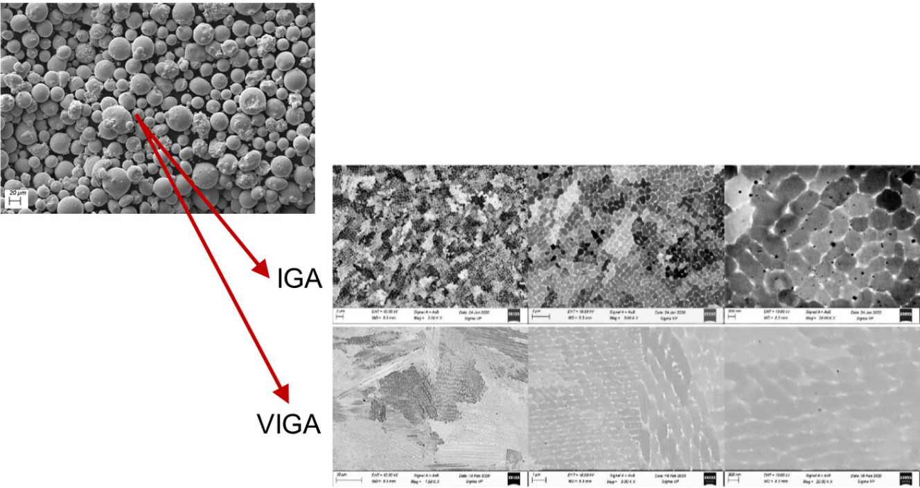
Figure 7: As-built microstructure of Inconel 718 (Source: Sandvik)
