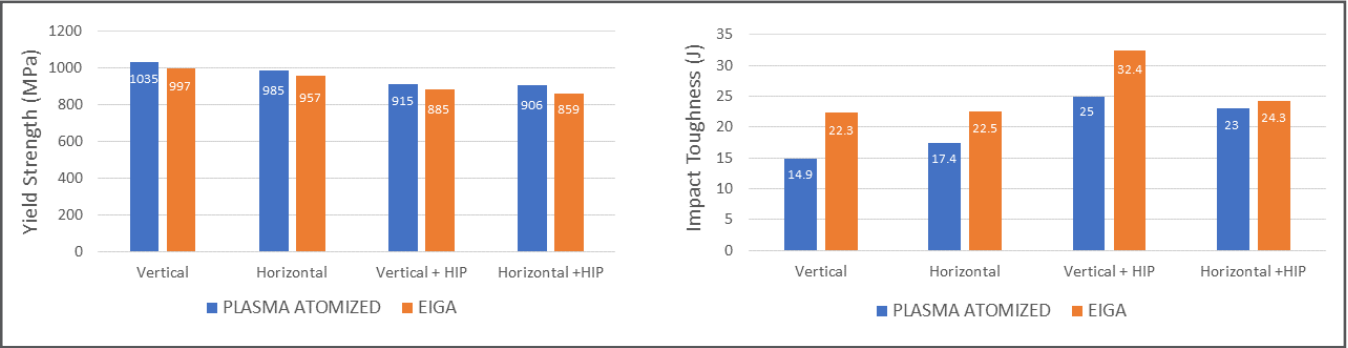
Figure 11: Mechanical Properties of Plasma atomized and EIGA type Ti6Al4V at 30μ (Source: Sandvik)
