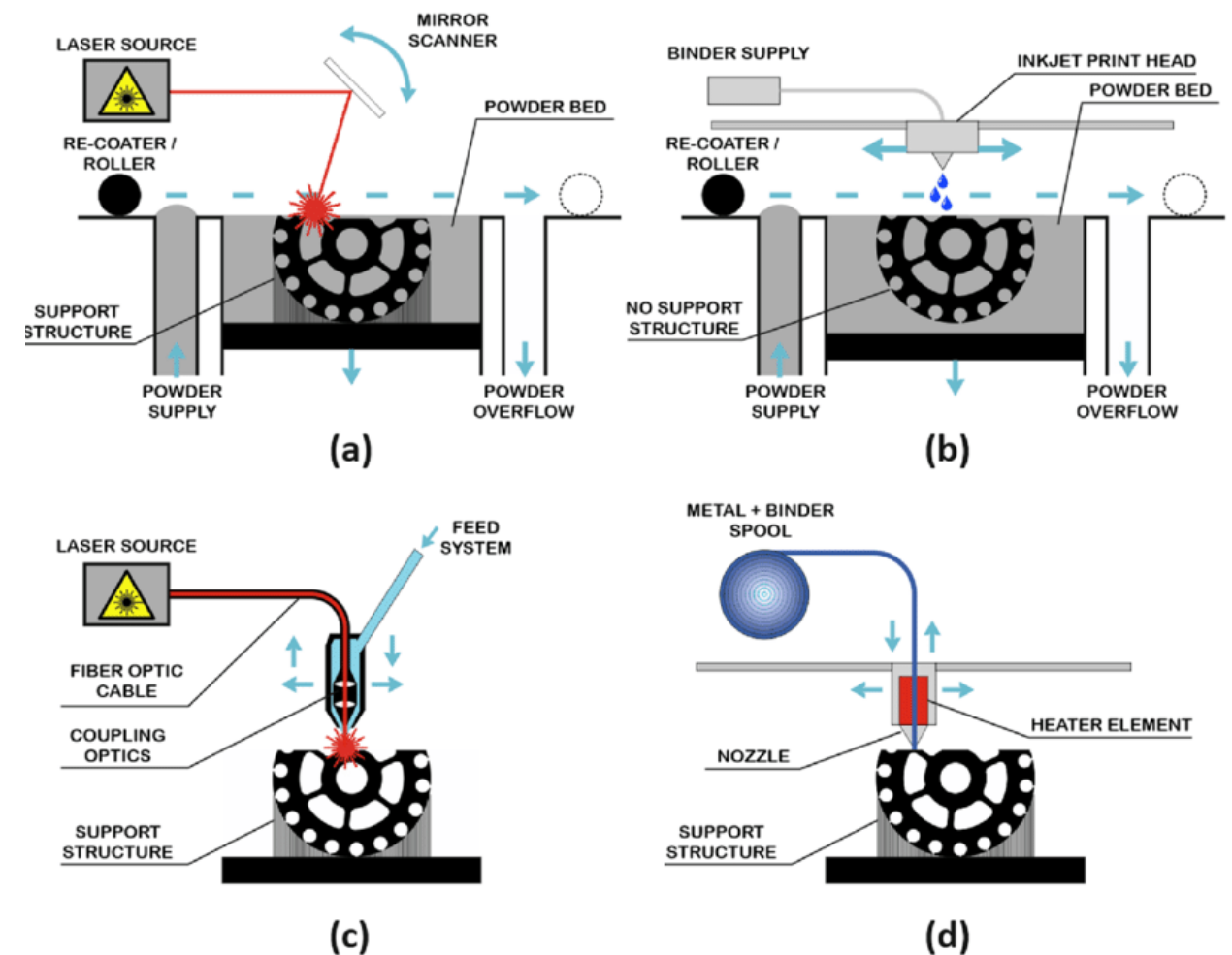
1. Common metal AM methods: (a) laser powder bed fusion (L -PBF), (b) binder jetting (BJ), (c) directed energy deposition (DED), (d) fuse deposition modelling (FDM).
