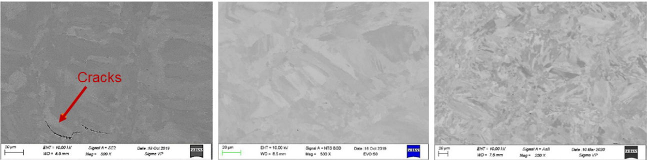
Figure 9: Microstructure of H-X alloy, as built – IGA standard composition (left), IGA optimised composition (middle), VIGA optimised composition (right) (Source: Sandvik)
