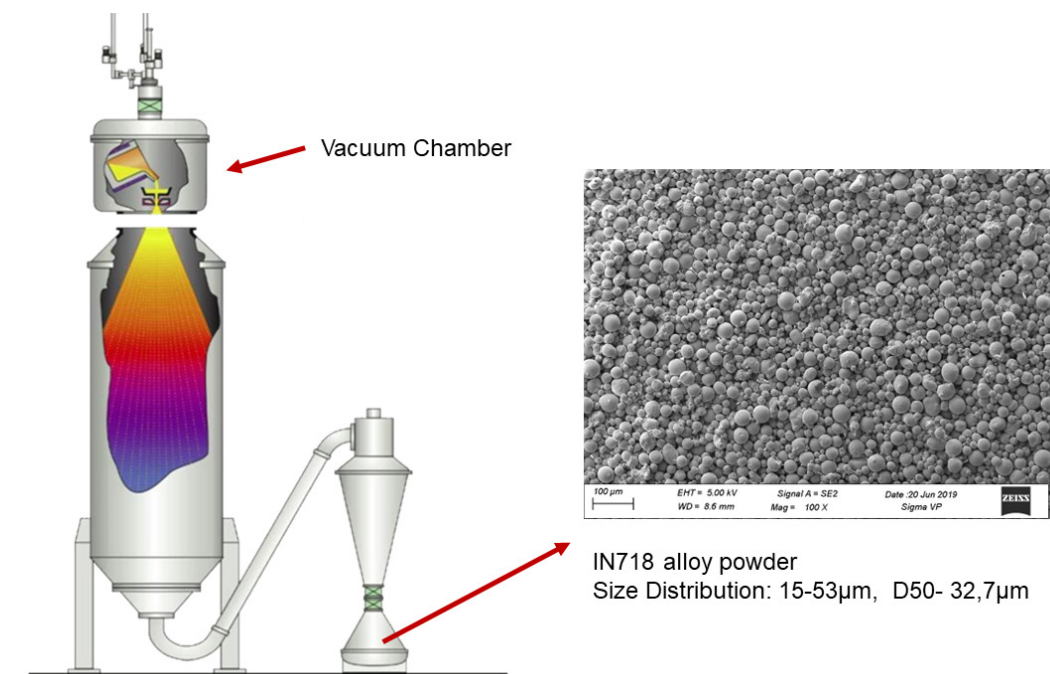
Figure 2: Vacuum Inert Gas Atomisation (Source: ALD Vacuum Technologies (left), Sandvik (right))
