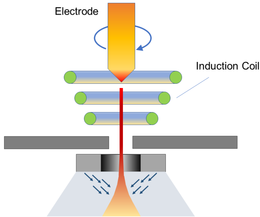
Figure 3: Electrode Induction Melting Inert Gas Atomisation (Source: ALD Vacuum Technologies)
