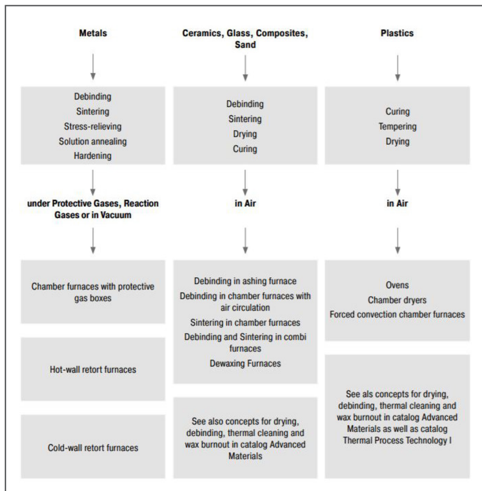
Source: Nabertherm – Heat Treatment of Additive Manufactured Parts
