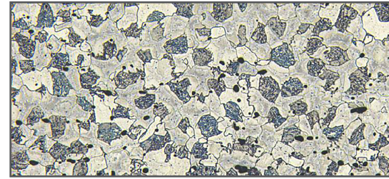
Legend: The cross-section of the FSLA material shows the dual-phase microstructure after heat treatment. Image: GKN Aerospace
